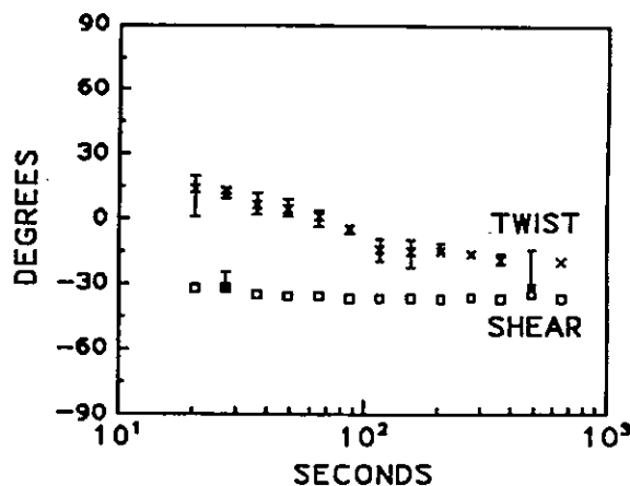
Fig. 5. Distortion parameters (twist and shear) for the interpretation given by Fig. 4
