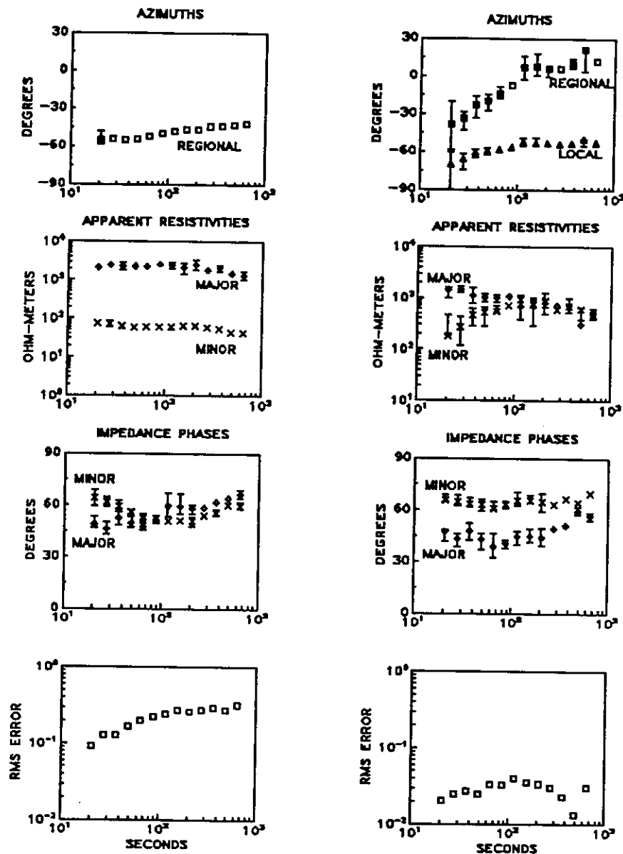
Fig. 4. Comparison of parameters by different methods. The left column contains graphs of the parameters, inductive strike, apparent resistivities, impedance phases, and error of fit by the conventional technique. The right column contains the same information by the new technique when the distortion parameters are not constrained to be independent of frequency.
