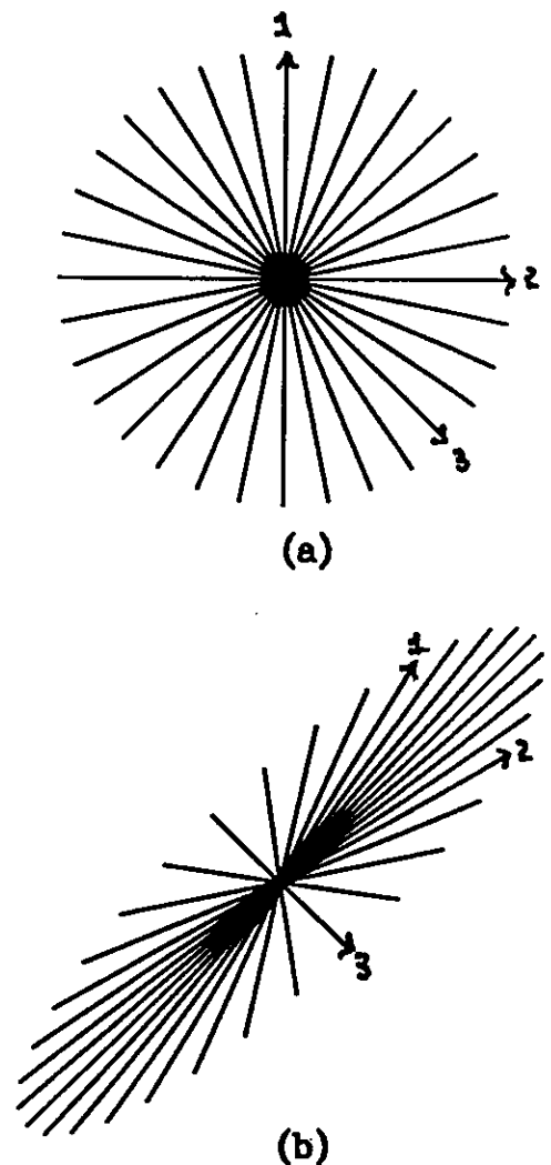
Fig. 3. A family of unit vectors (a) before and (b) after the application of the shear tensor S . The x axis is up, the y axis to the right.
