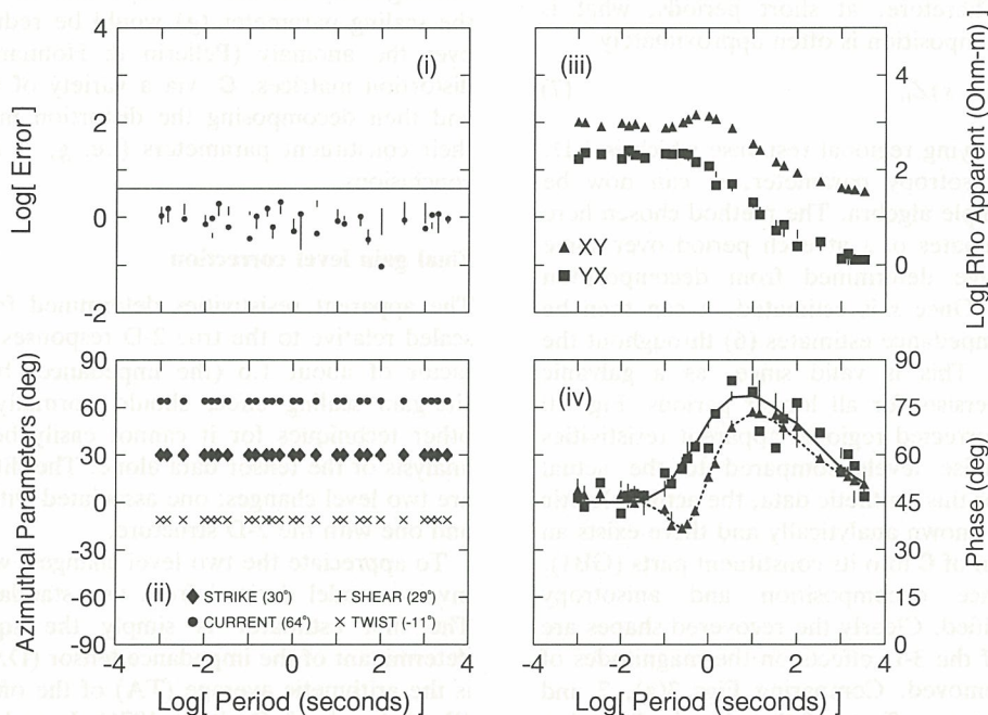
Figure 9. The residual error, strike, twist and shear, and regional impedance estimates for a constrained 3-D model parameterization of 3-D data with (2 per cent) noise. True regional phase responses are given for comparison.
