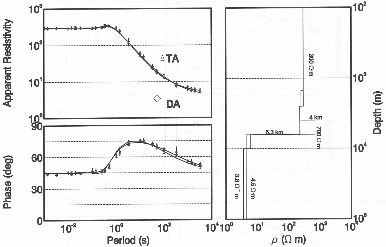
Figure 11. 1-D resistivity and phase responses (left panels) for the minimum structure inverse model from DA (bold line) and TA estimates for the true regional response plus noise.
