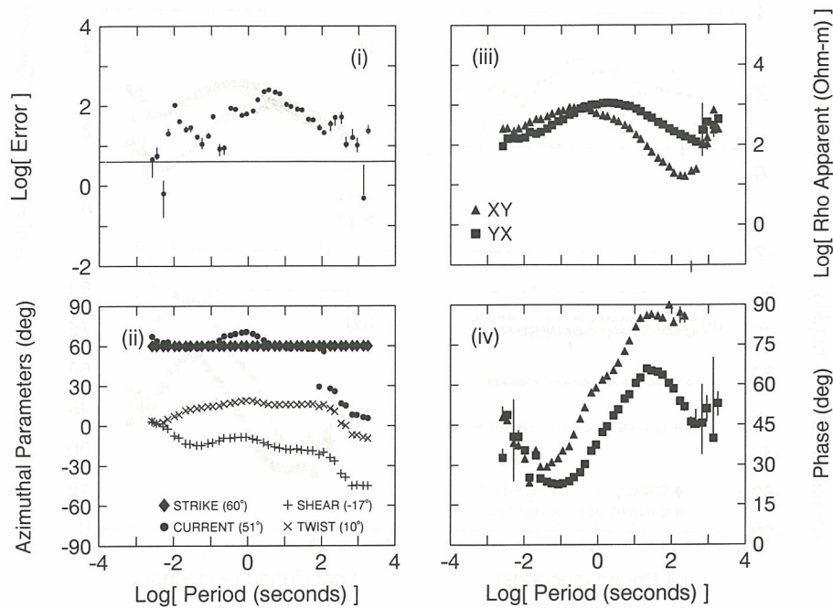
Figure 18. The 3-D model parameters for field data from site LITW02 with strike constrained to 60°.
