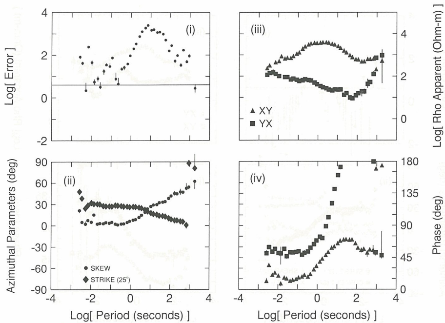
Figure 20. The 2-D model parameters for field data (LIT000) for best fitting strike.
