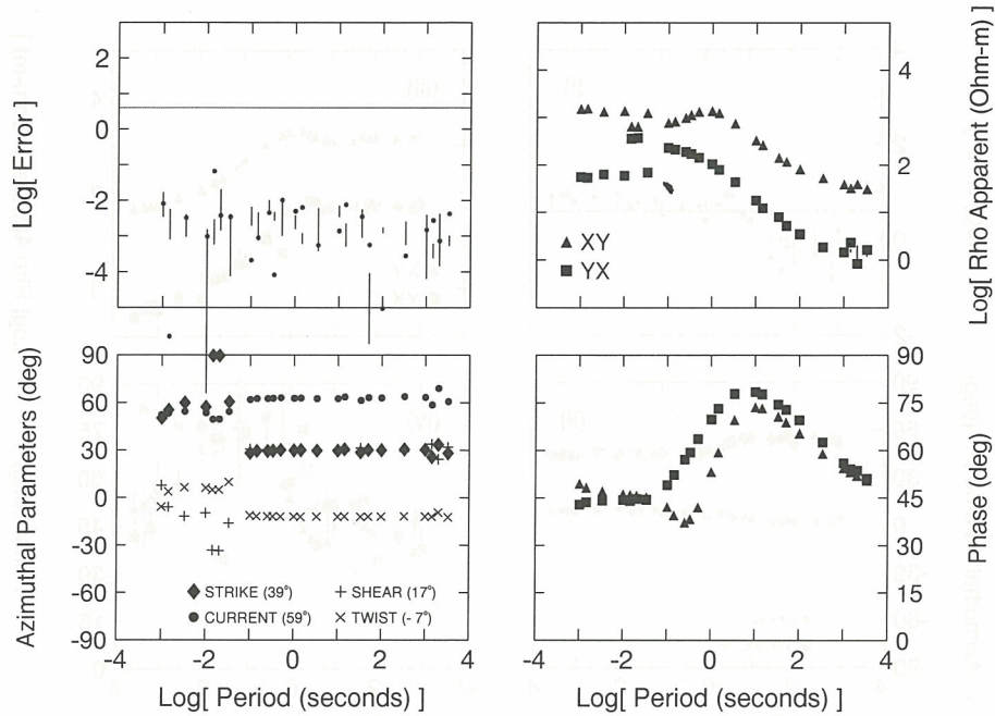
Figure 6. The residual error, strike, twist and shear, regional impedance estimates and channelling azimuth for an unconstrained 3-D model parameterization of 3-D data with 0.1 per cent noise.
