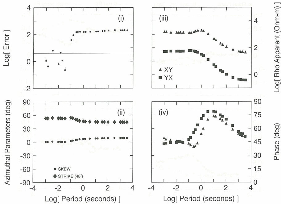
Figure 3(a). The residual error (i), strike, skew (ii), and regional apparent resistivity and phase (iii, iv) estimates for a 2-D model parameterization of the synthetic 3-D data with 0.1 per cent noise.
