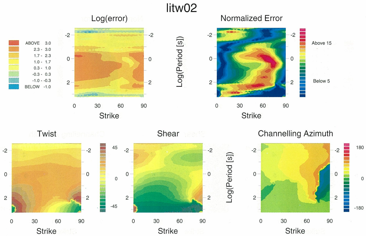
Figure 17. The chi-squared residual, normalized residual and distortion parameters for a 3-D parameterization of the data from site LITW02 as a function of regional strike and period.
