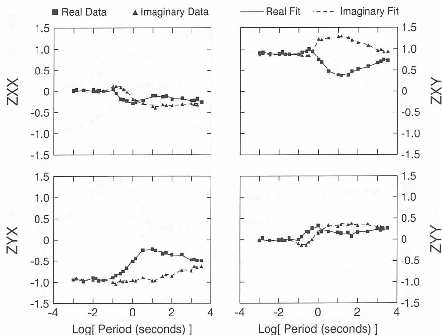
Figure 2(b). Fit of the model parameterization of Fig. 2(a) to the scaled impedance data (see text for details). Error bars indicate one standard deviation of the data. Square symbols and solid lines represent in-phase data and model impedance. Triangular symbols and dashed lines represent quadrature data and model impedance.
