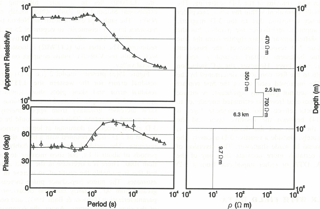
Figure 13. Decomposition Trace (DTA) for synthetic 3-D data and 1-D model responses (left panel) for the resistivity model (right panel) determined by a minimum structure inversion.
