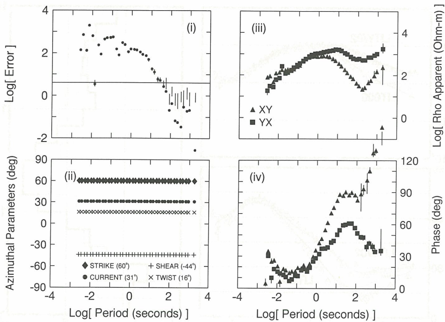
Figure 25. Final model parameters after correction for anisotropy in apparent resistivities for site LIT000.
