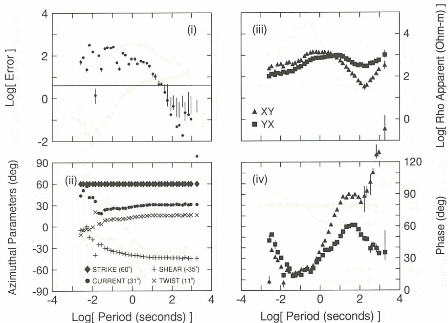
Figure 24. The 3-D model azimuthal parameters and residual for field data (LIT000) for strike constrained to 60°
