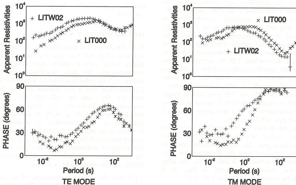
Figure 26. Comparison of recovered regional TE and TM mode responses after anisotropy corrections for stations LITW02 and LIT000.
