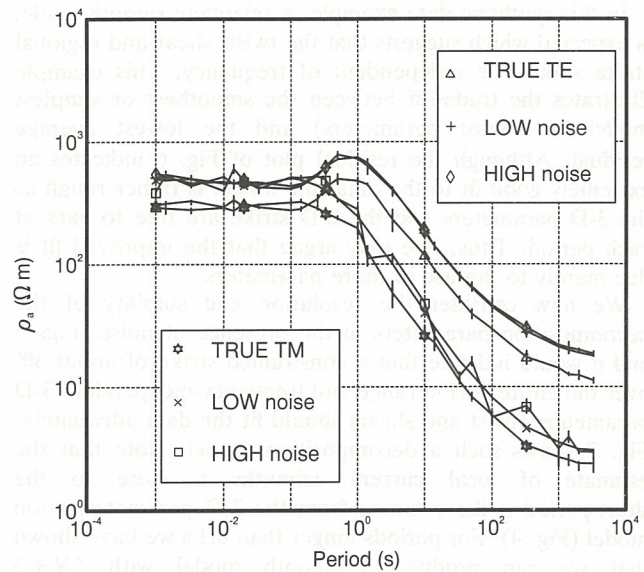
Figure 10. Comparison of estimated regional apparent resistivities after anisotropy correction. Low noise 0.1 per cent. High noise 2 per cent.
