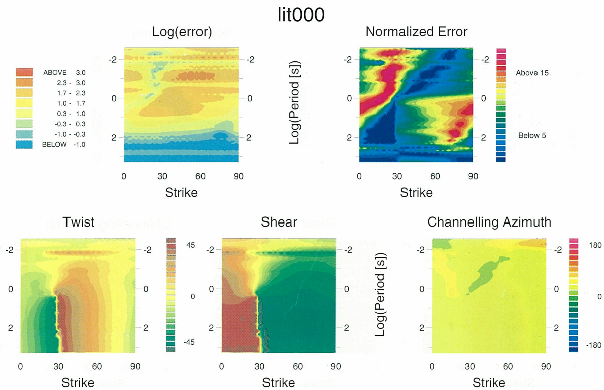
Figure 23. The chi-square residual, normalized residual and distortion parameters for a 3-D parameterization of the data from site LIT000 as a function of regional strike and period.
