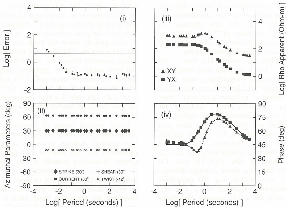
Figure 7. The residual error, strike, twist and shear, regional impedance estimates for a fully constrained 3-D model parametrization of 3-D data with 0.1 per cent noise. The solid and dashed lines show the true 2-D phase responses (Fig. 2) parallel and perpendicular to the regional strike.
