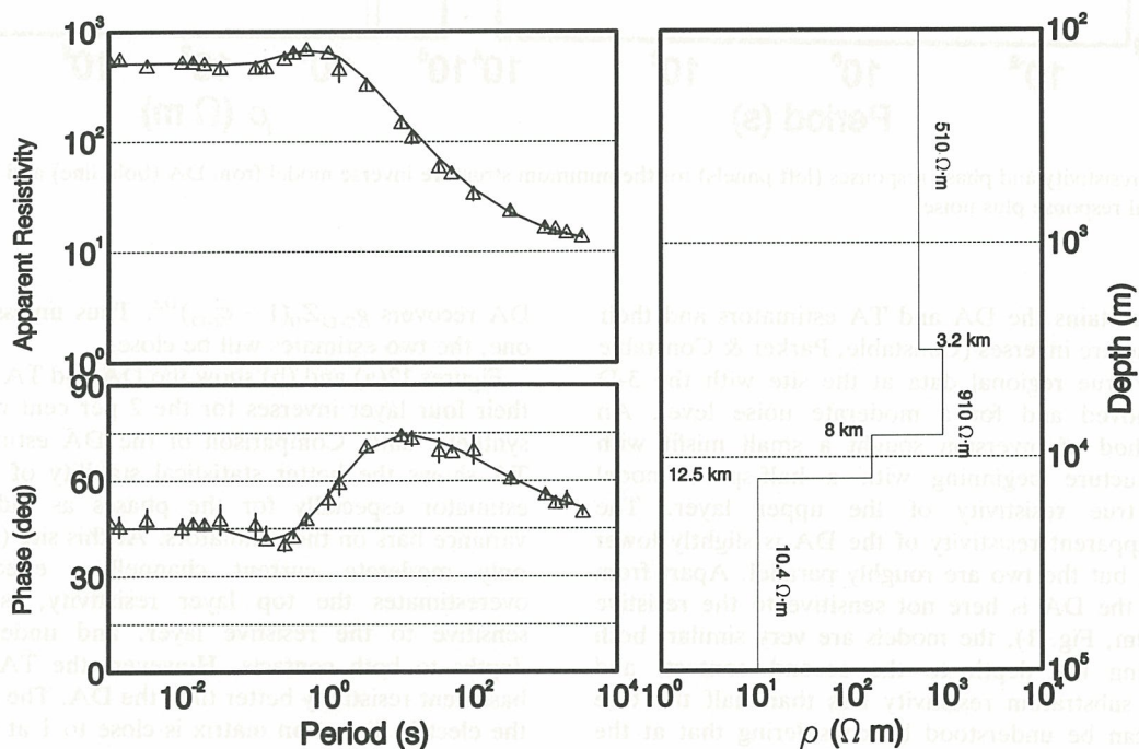
Figure 12(b). Inverse of anti-trace average (TA) for same data.
