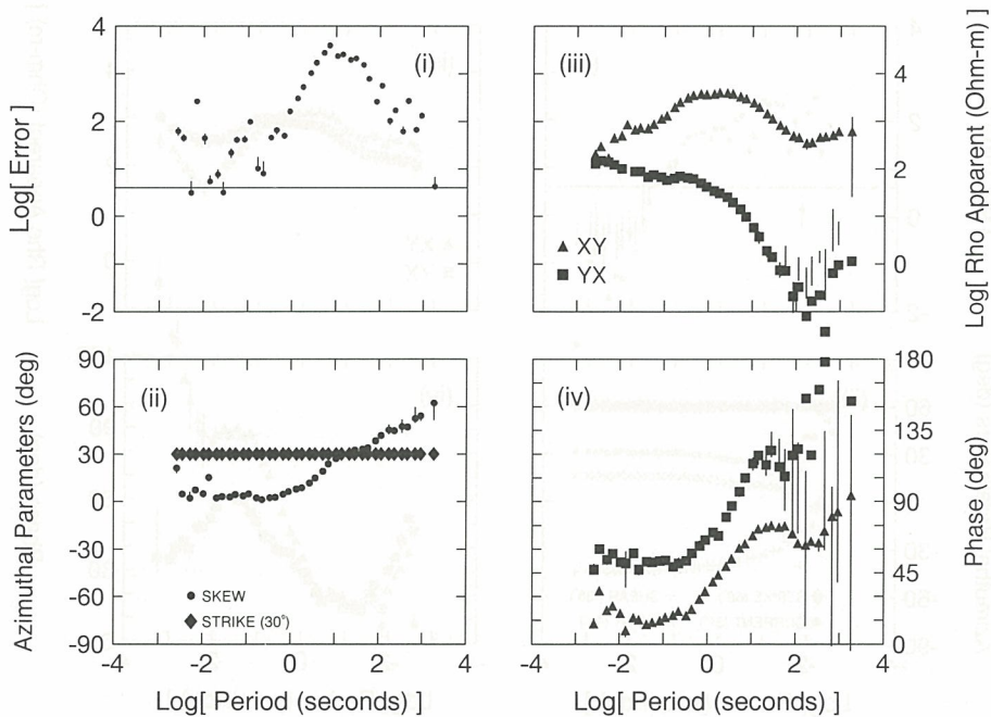
Figure 21. The 2-D model parameters for field data (LIT000) with strike constrained to short-period 2-D strike azimuth (30°).
