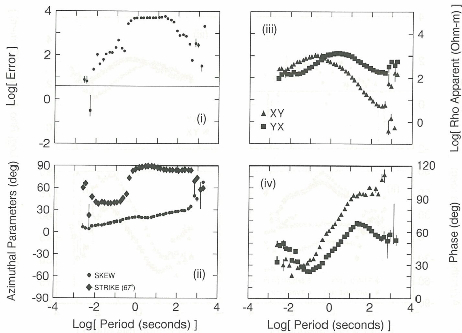
Figure 15(a). The 2-D model parameters for field data from station LITW02 for best fitting strike.
