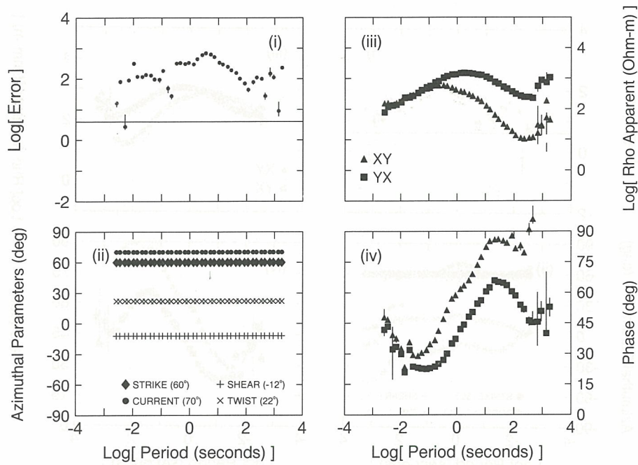
Figure 19(a). The 3-D model parameters for field data from site LITW02 for a fully constrained model after correction for anisotropy in apparent resistivities.
