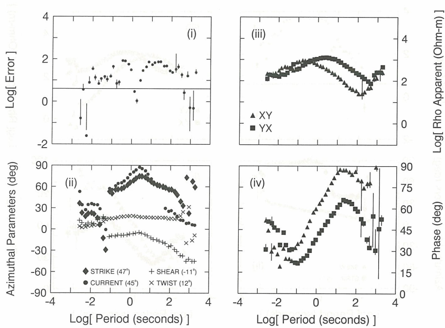
Figure 16(a). The unconstrained 3-D model parameters for field data from station LITW02.
