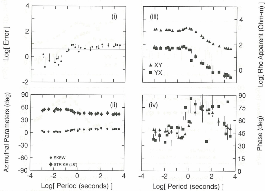
Figure 4. The residual error, strike, skew, regional impedance estimates for a 2-D model parameterization of 3-D data with 2 per cent noise.
