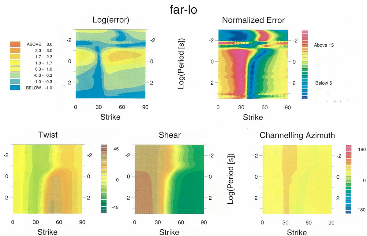
Figure 5. The logarithm of the residual error, the relative or normalized error, the twist and shear angles, and an estimate of local current polarization azimuth (channelling azimuth) for synthetic 3-D data with 0.1 per cent noise contoured as functions of strike angle and period (see text for details).
