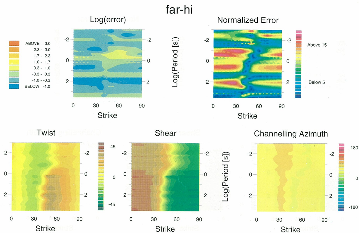
Figure 8. The chi-square residual error, normalized error, twist and shear angles and channelling azimuths for synthetic 3-D data with 2 per cent noise as functions of strike angle and period.
