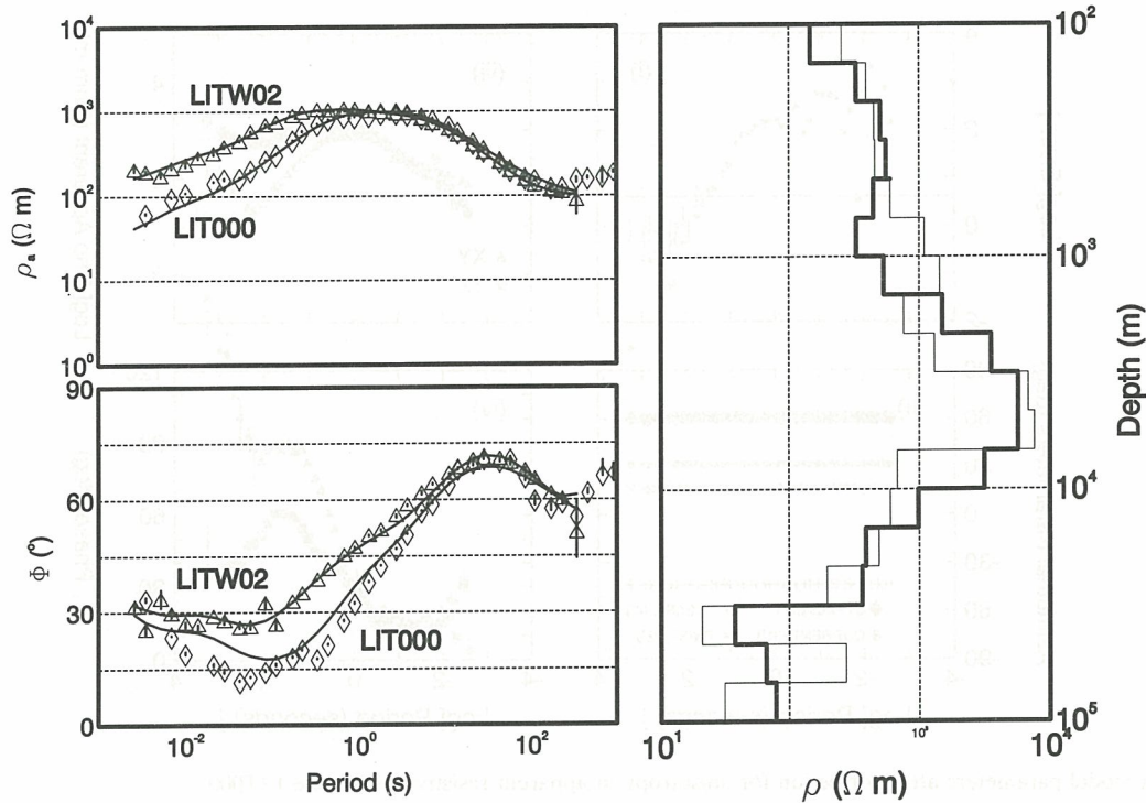
Figure 27. DTA estimators for stations LITW02 (bold response and model lines) and LIT000 with smooth minimum-structure inverses.
