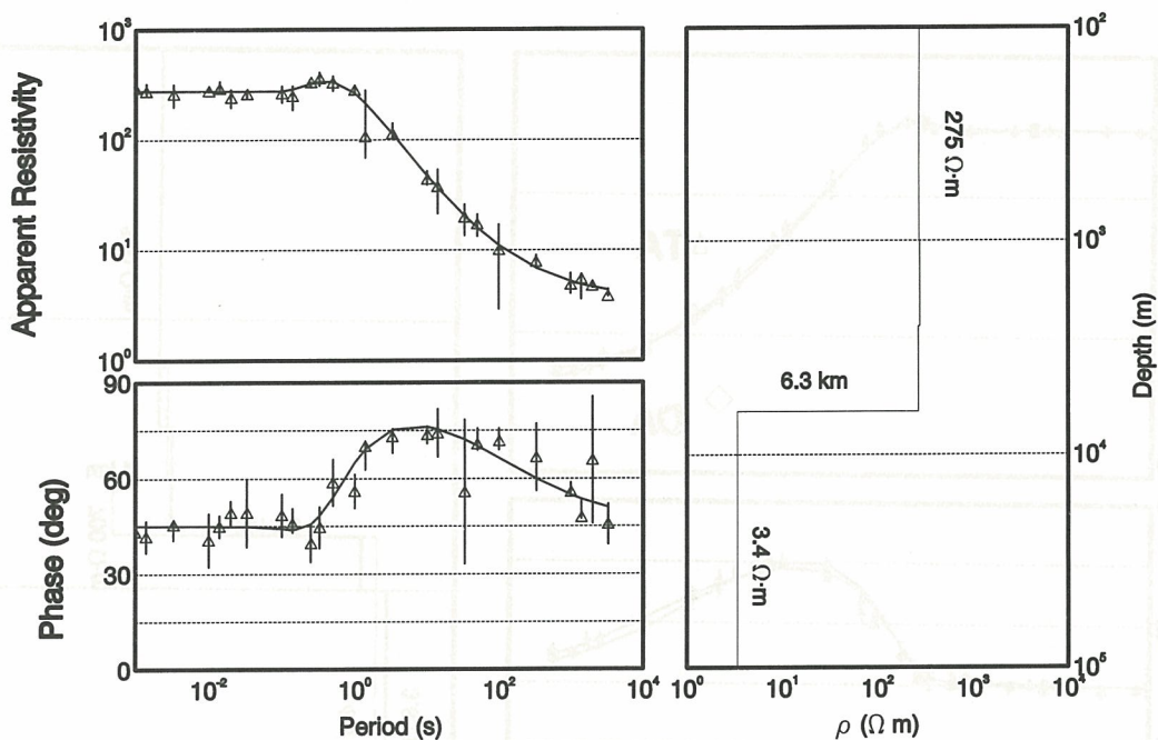
Figure 12(a). Minimum structure 1-D inverse of determinant average (DA) of 3-D synthetic data with (2 per cent) noise.
