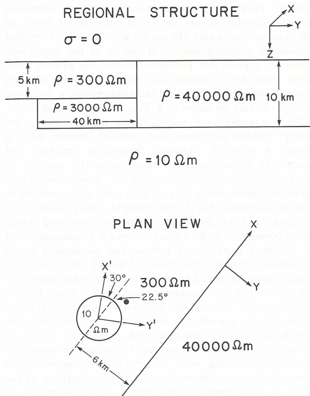
Figure 1. The synthetic regional 2-D conductivity structure (GB2) not to scale. The measurement site is indicated. The hemisphere has a 50 m radius and is located 6 km from the vertical contact in the 2-D model. The measurement axes labelled x' and y' are rotated 30^\circ anticlockwise from the 2-D intrinsic co-ordinate system (strike based).
