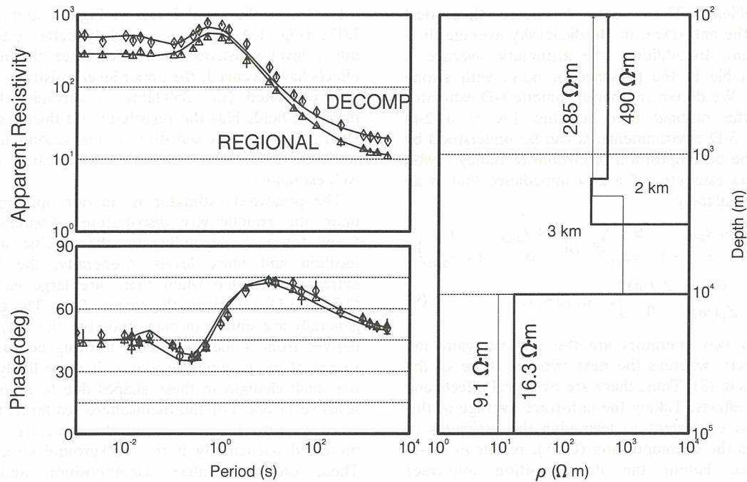
Figure 14. Comparison of the true regional TE 1-D inverse to estimated regional TE inverse after all 3-D corrections. In the right panel, the bold line represents the model from the 3-D data after decomposition.
