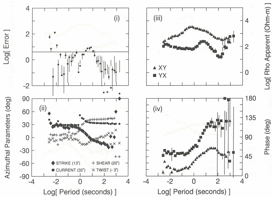
Figure 22. The unconstrained 3-D model parameters for field data (LIT000).
