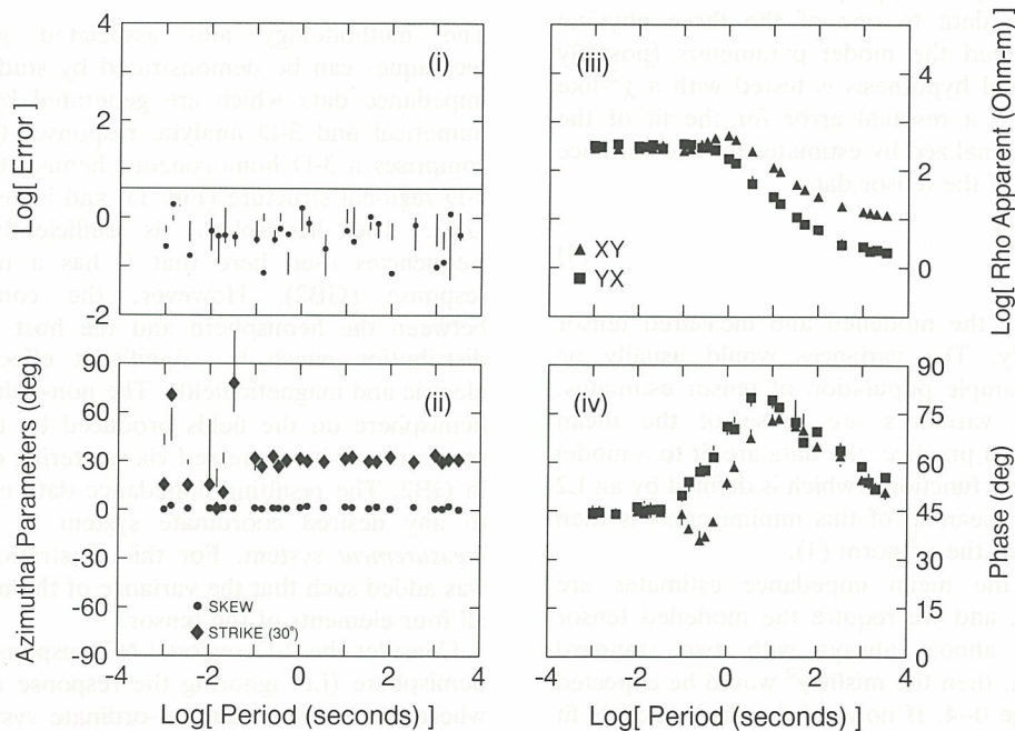
Figure 2(a). Standard parameter display. (i) Residual error of the fit of the model to the data, (ii) azimuthal parameters (strike and skew), (iii) estimated regional apparent resistivities in strike azimuth, (iv) estimated regional phases. The parameters are calculated for 2-D synthetic data (including 3 per cent noise), which were rotated to the measurement system. The values given at the bottom of the 'Azimuthal Parameters' plot are the average values for these parameters over the entire period band.
